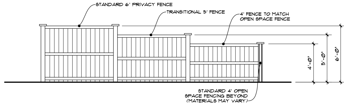
ELEVATION VIEW
